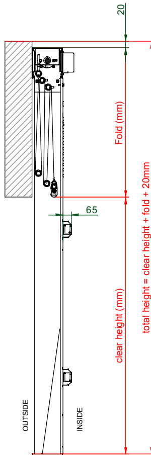
INDOOR INSTALLATION
